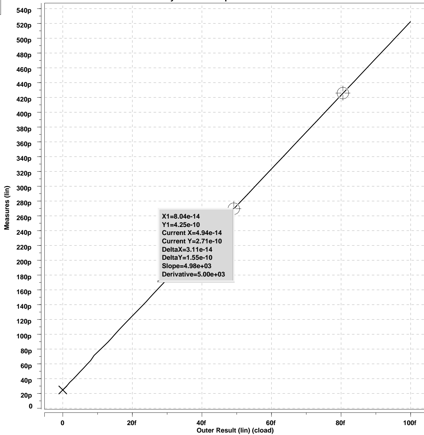
hw5#1b delay with load capacitance 0 to 100ff
