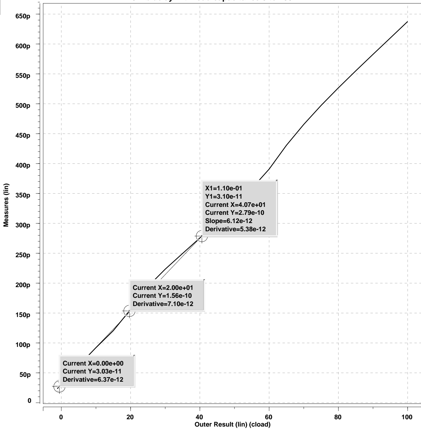
hw5#1b delay with load capacitance 0 to 100ff
